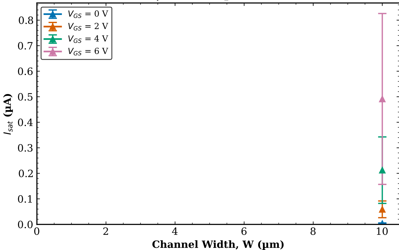
TFT3 Combined (Tr. 1 & 2) I_{sat} vs W | L = 160\text{ }\mu\text{m} (mean \pm std)
